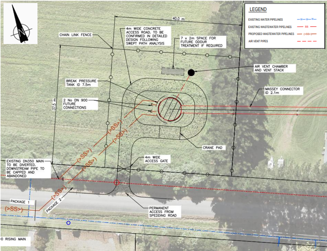
Figure 1. Break Pressure Tank Site Layout 8 Spedding Road
