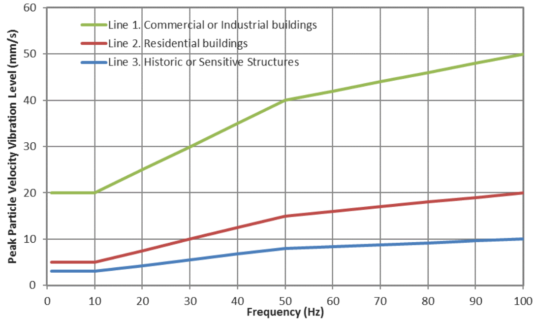
Figure 5: Short-term (transient) vibration at building foundations (DIN 4150-3 1999: Figure 1)
