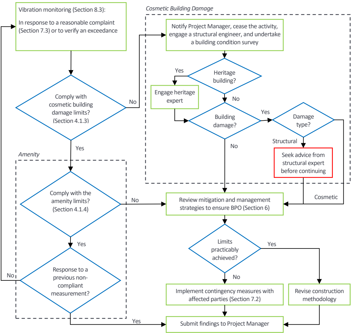
Figure 7: Vibration Monitoring Flow Chart
