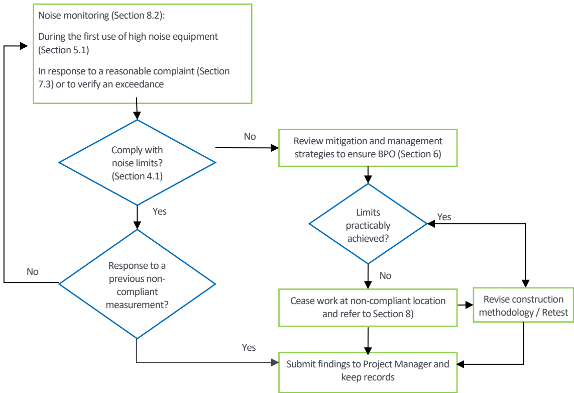
Figure 6: Noise Monitoring Flow Chart
