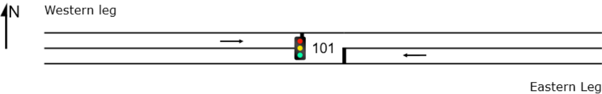
Figure 4-8: Site Layout of 1-lane 2-way Operation on Brigham Creek Road
