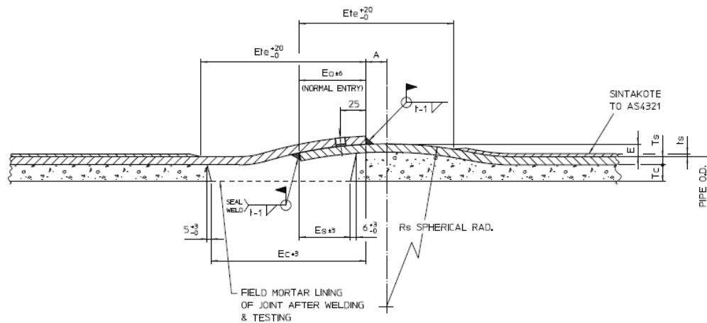
Figure 1: Spigot and socket joint illustration.
