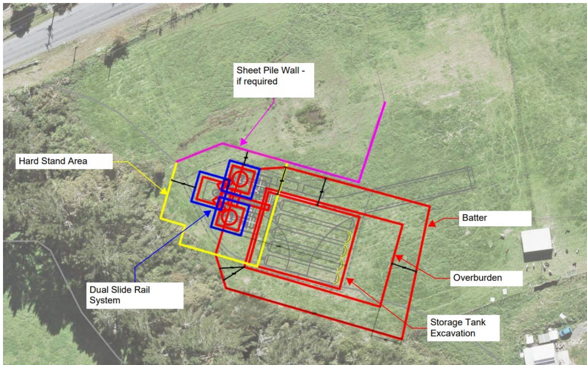
Figure 23. Overall schematic of earthworks
