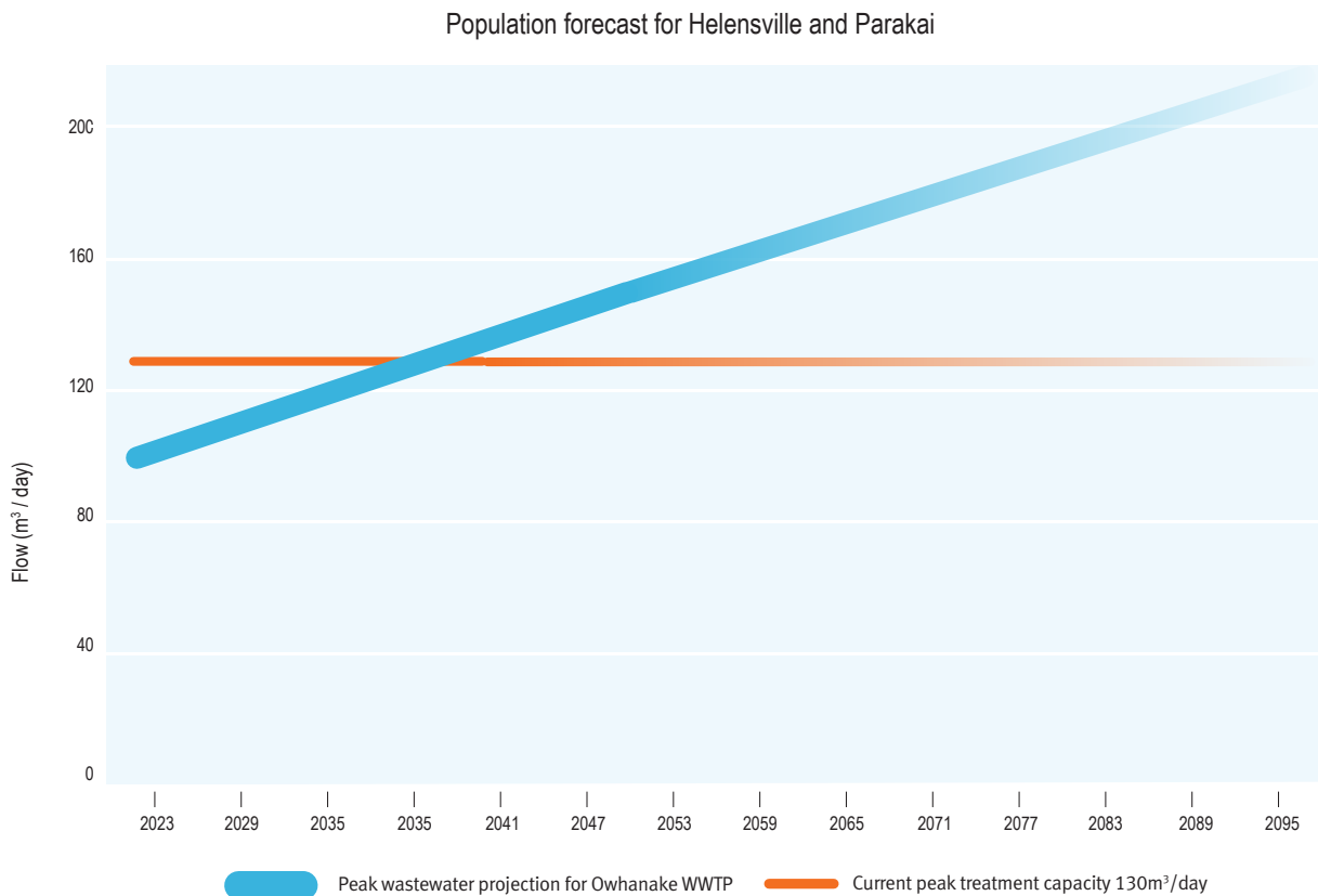
Figure 12 – Projected peak wastewater flows to Owhanake treatment plant based on the high-growth projection for Auckland population
